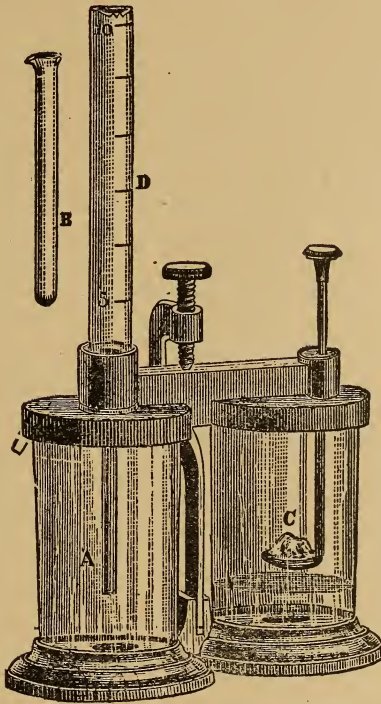
Fig. 71. TWICHELL'S APPARATUS FOR DETERMINING THE STRENGTH OF VINEGAR.
